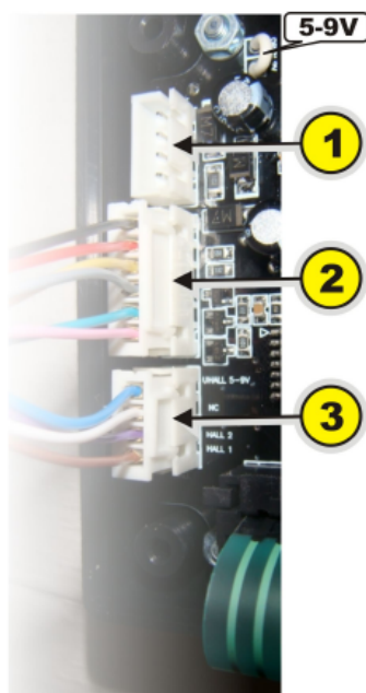
Picture 1. Connectors.
